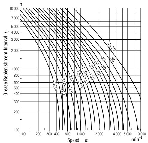
(2) Tapered Roller Bearings, Spherical Roller Bearings
