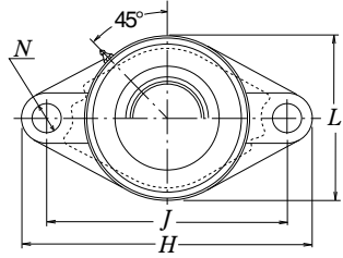
Pressed steel dust cover type Open end Z-UCFL...D1 Closed end ZM-UCFL...D1
