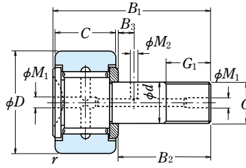
Full Complement
