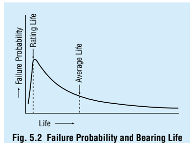
Fig. 5.2 Failure Probability and Bearing Life
