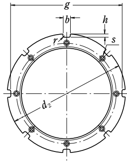
Nut with Stopper
