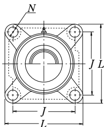
Pressed steel dust cover type
