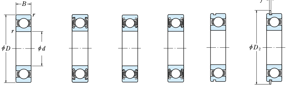
Open Type
