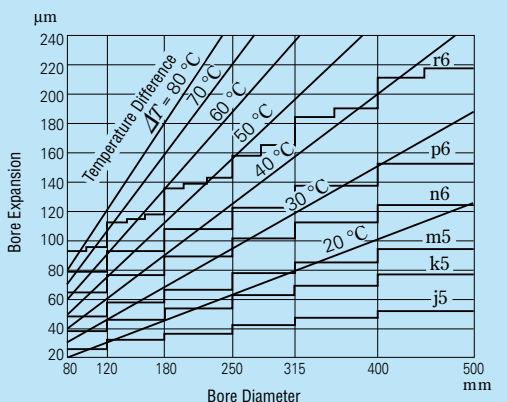
Fig. 14.3 Temperature and Thermal Expansion of Inner Ring
