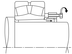
Fig. 14.17 Removal of Withdrawal Sleeve Using Withdrawal Nut (2)
