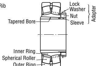
Spherical Roller Bearing
