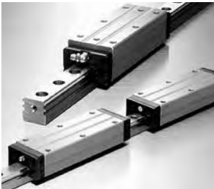
NSK Linear Guides High-Accuracy Series (CAT. No. E3329, E3162)
