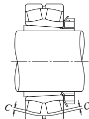
Fig. 14.8 Clearance Measurement of Spherical Roller Bearing
