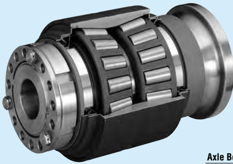
Axle Bearings
