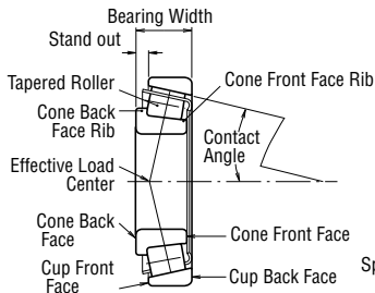
Tapered Roller Bearing
