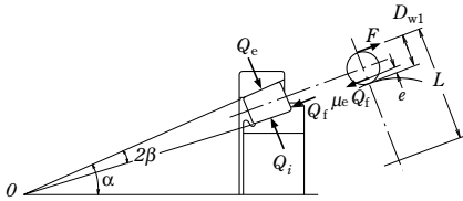
Fig. 15.9 Relation between e and \beta
