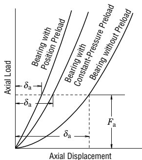
Fig. 10.6 Comparison of Rigidities and Preloading Methods
