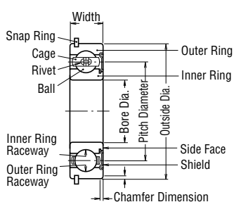
Single-Row Deep Groove Ball Bearing
