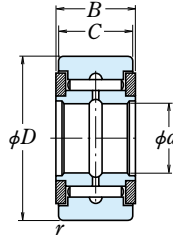
Full Complement
