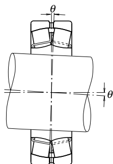
Fig. 3.4 Permissible Misalignment of Spherical Roller Bearings
