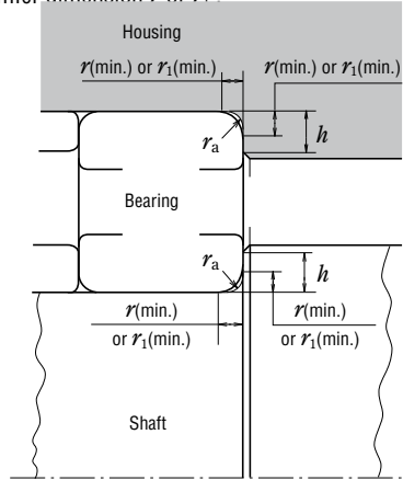
Fig. 11.1 Chamfer Dimensions, Fillet Radius of Shaft and Housing, and Shoulder Height
