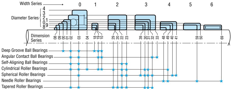
Fig. 3.1 Dimension Series of Radial Bearings
