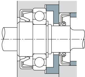
Fig. 11.8 Example of Application of Oil Seal (1)
