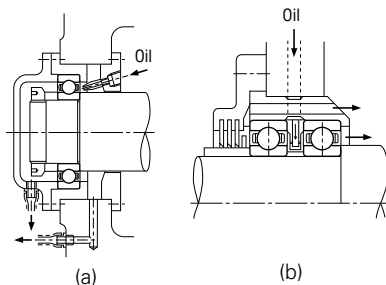
Fig. 12.8 Jet Lubrication
