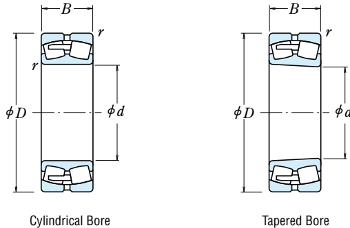
Cylindrical Bore
