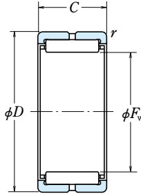
Without Inner Ring RNA
