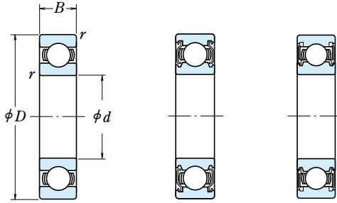
Shielded Type ZS
