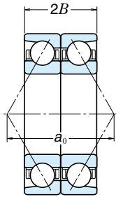
Back-to-Back DB
