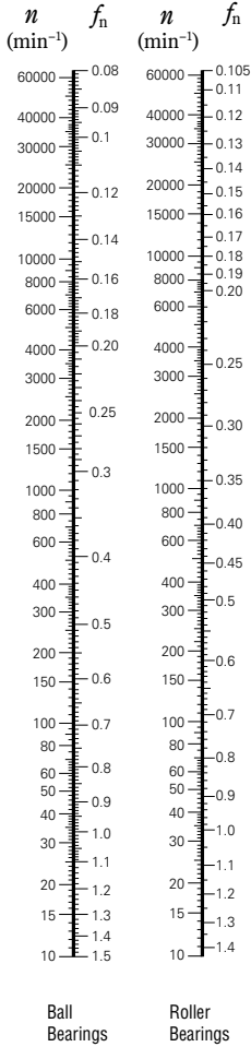
Fig. 5.3 Bearing Speed and Speed Factor
