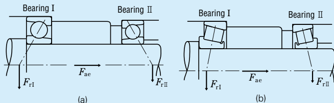
Fig. 5.12 Loads in Opposed Duplex Arrangement
